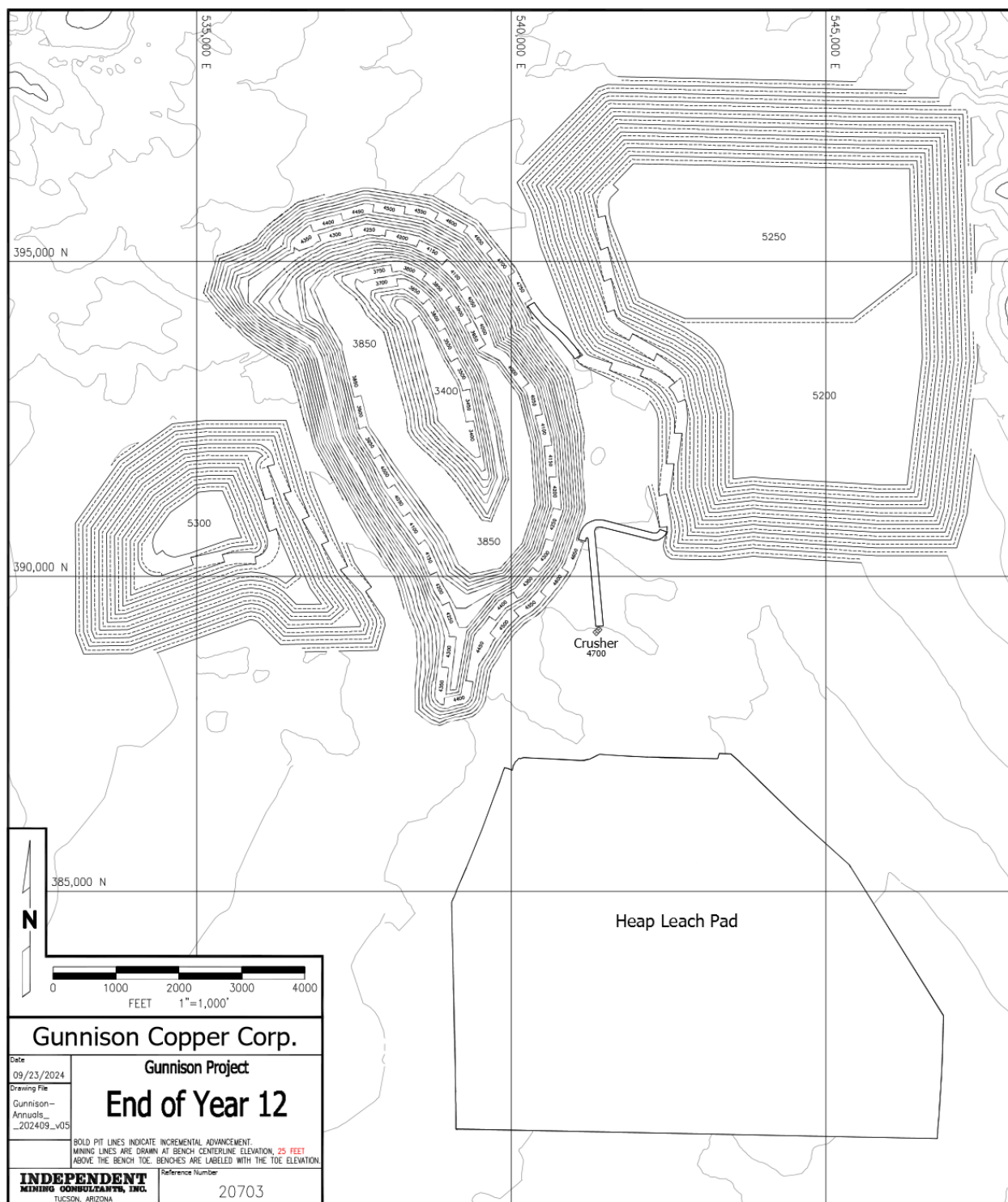
Figure 16-10: Pit and Dump Configuration at the end of Year 12 of Mining
