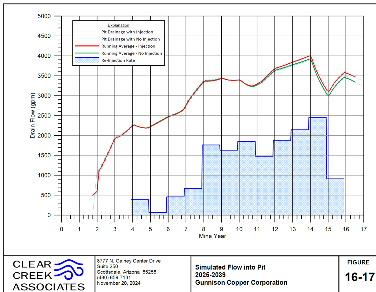
Figure 16-17: Simulated Flow into Pit
