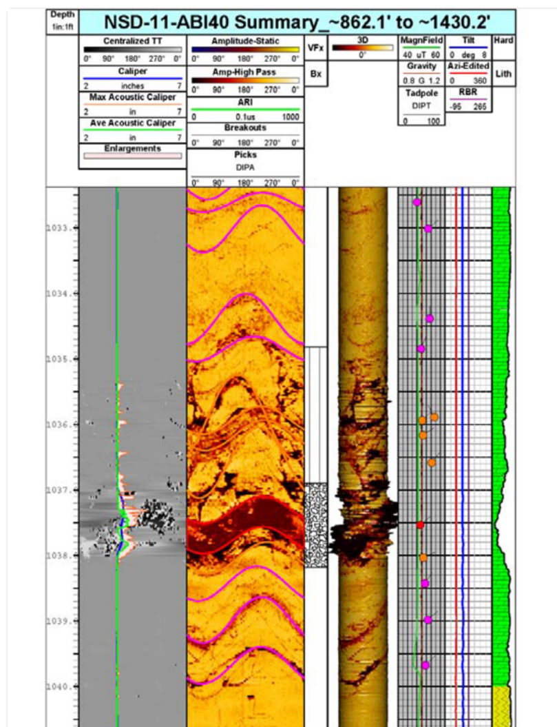
Figure 9-1: Graphical Example of Geophysical Log
