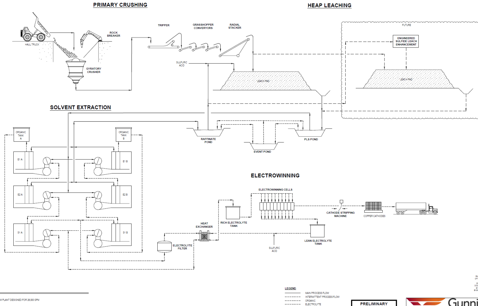
Figure 17-1: Overall Process Flow Diagram
