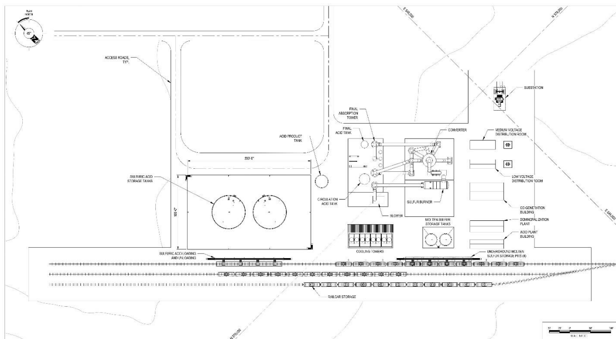
Figure 18-6: Sulfuric Acid Plant and Railyard
