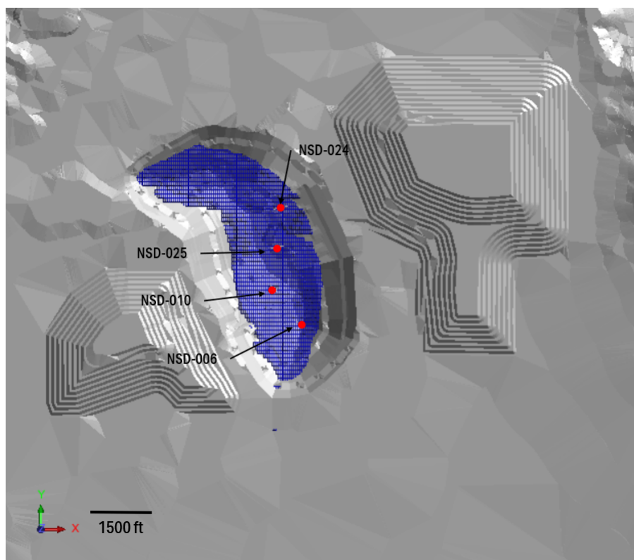
Figure 24-2: Drillhole Locations
