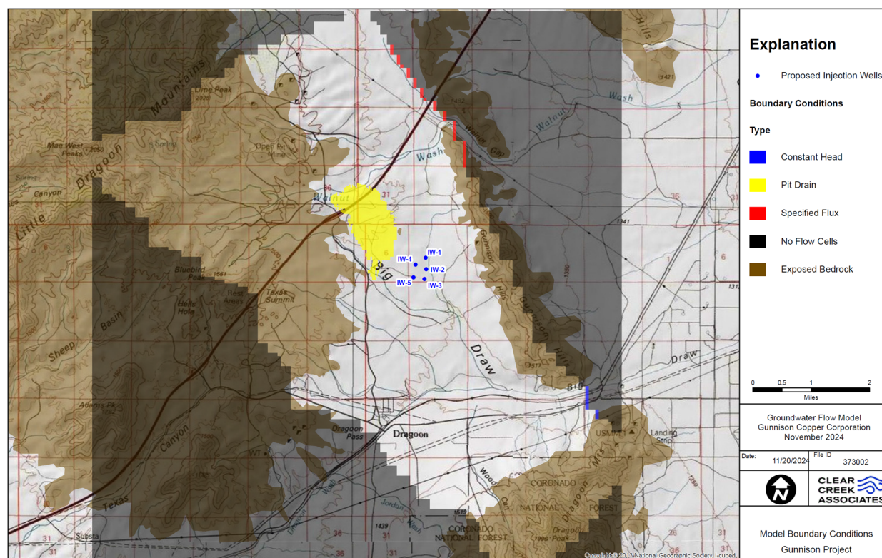
Figure 16-15: Groundwater Flow Model
