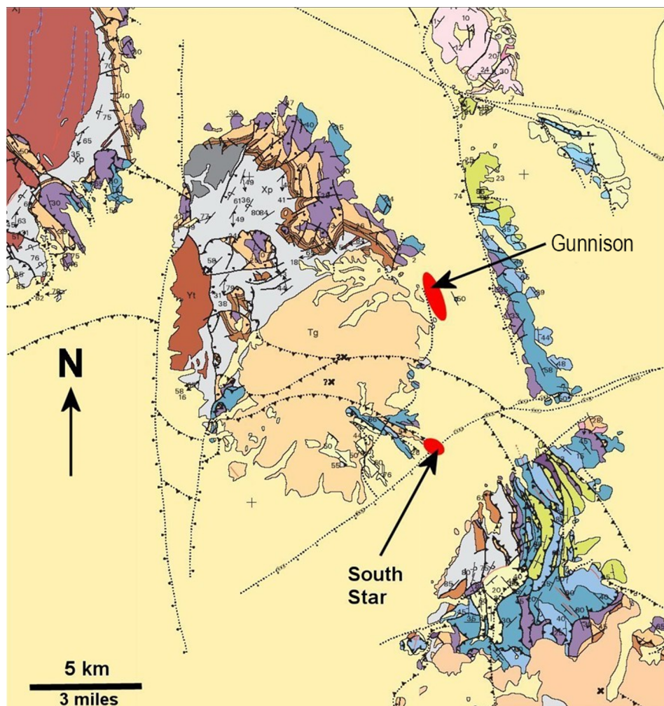
Figure 7-2: Geologic Map of the Little Dragoon Mountains (Modified from Drewes et al, 2001)
