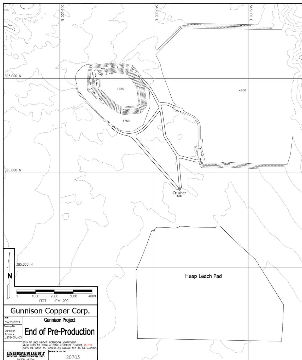
Figure 16-4: Pit and Dump Configuration at the end of Pre-Production Mining
