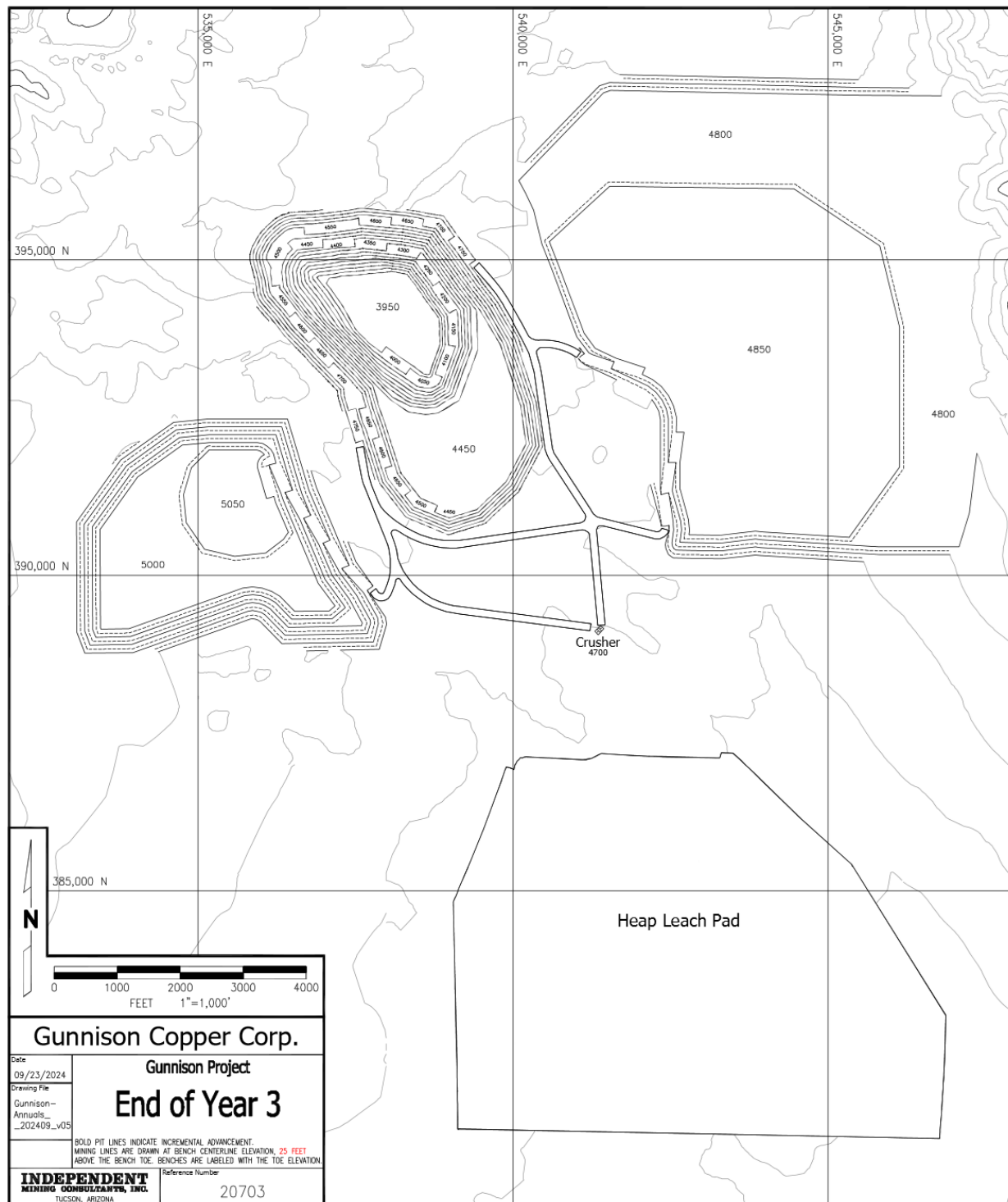
Figure 16-7: Pit and Dump Configuration at the end of Year 3 of Mining
