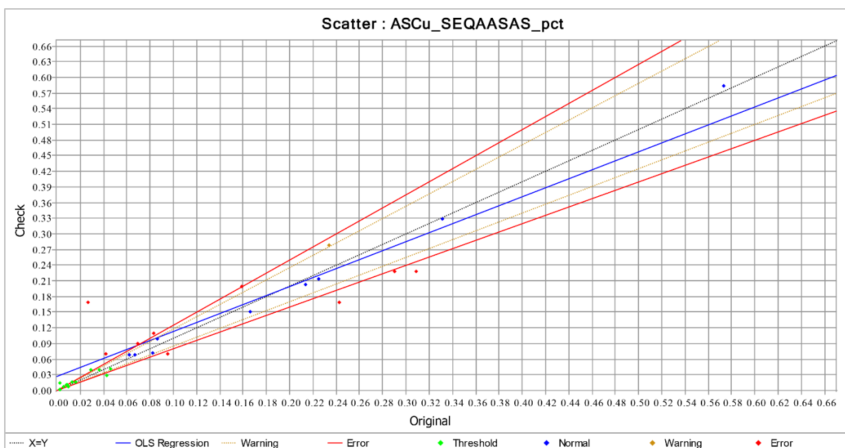
Figure 11-11: 2022 Field-Duplicate Acid-Soluble Copper (“ASCu”) Results Relative to Primary Sample Assays
