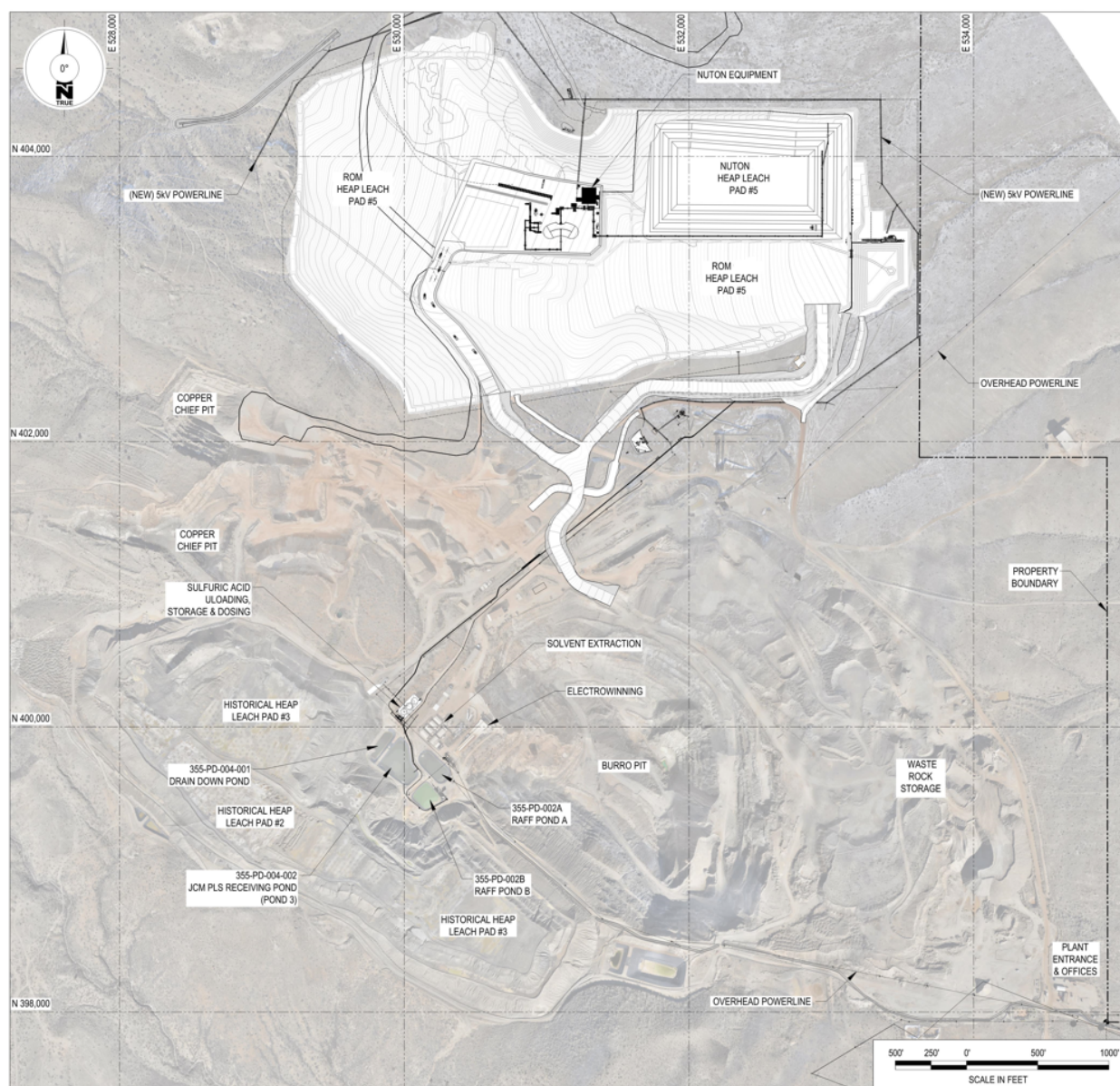
Figure 18-1: Johnson Camp Mine Facilities
