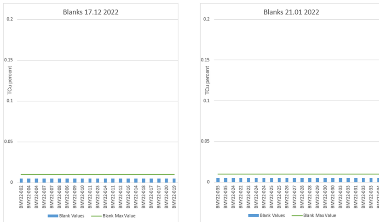
Figure 11-9: 2022 Coarse Blank Copper Values
