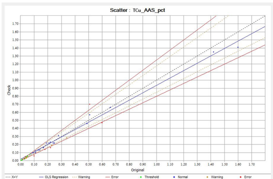
Figure 11-4: 2016 – 2017 Core-Duplicate Total Copper (“TCu”) Results Relative to Primary Sample Assays
