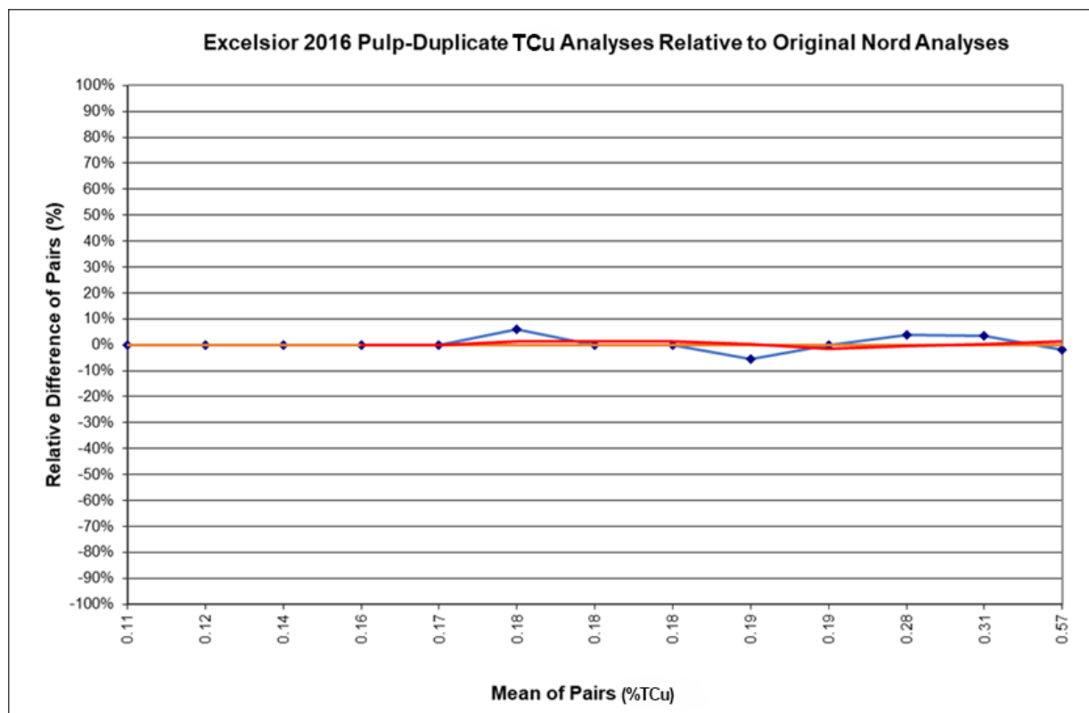
Figure 12-9: 2016 Total Copper ("TCu") Pulp-Duplicate Analyses Relative to Historical Nord Analyses
