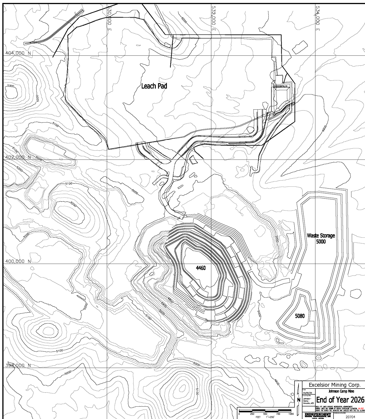
Figure 16-2: Pit and Dump Configuration at the end of 2026
