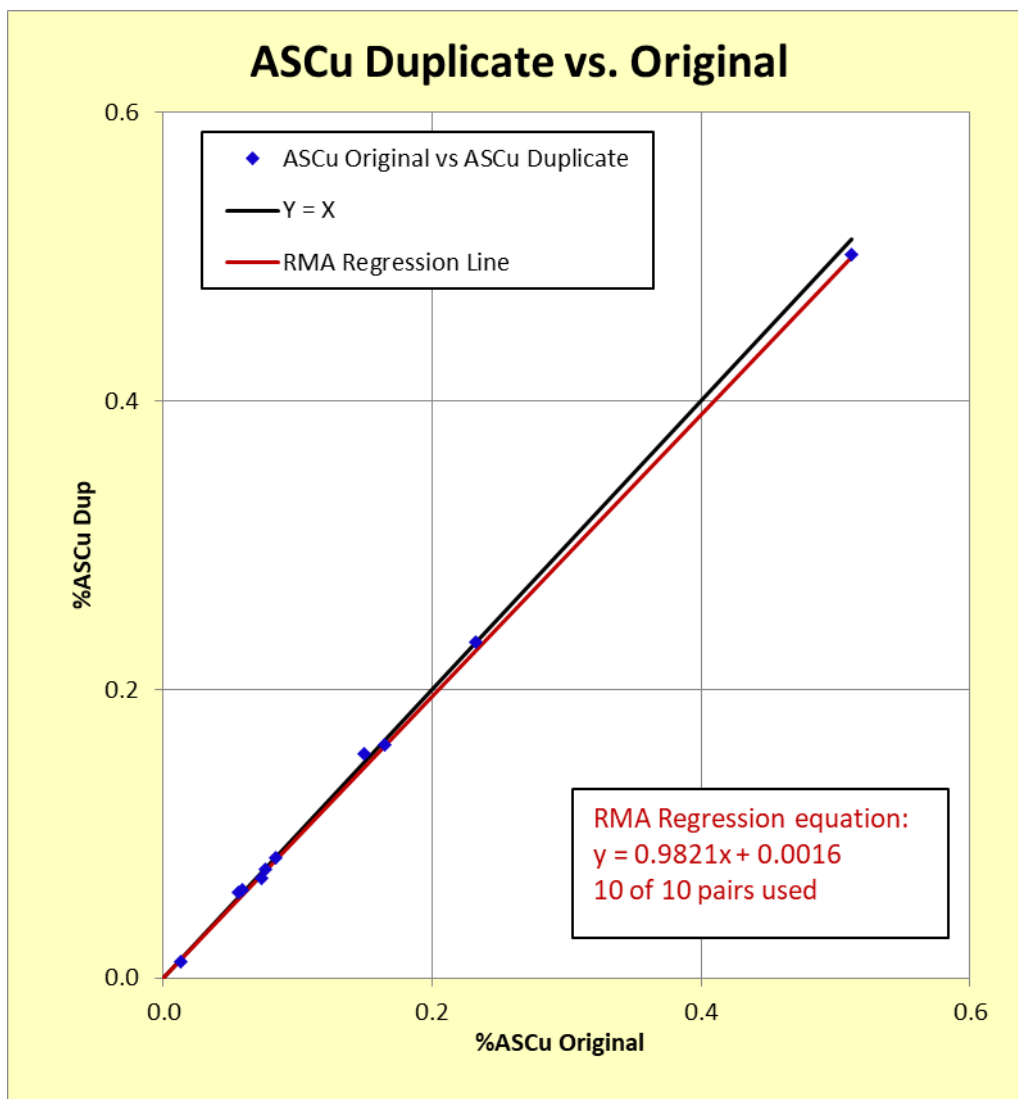
Figure 11-33: 2024 Pulp-Duplicate Acid-Soluble Copper (“ASCu”) Results Relative to Primary Sample Assays
