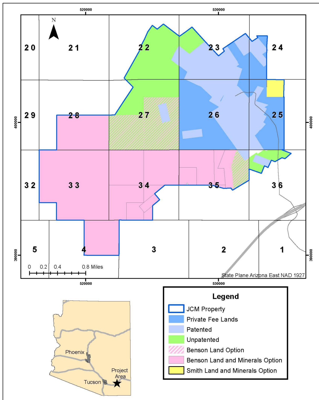
Figure 4-2: Property Mineral Rights by Claim Type – January 2025
