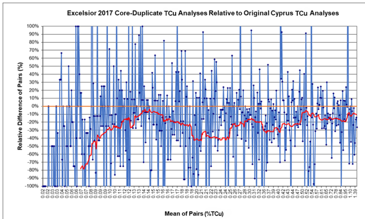
Figure 12-6: 2017 Total Copper (TCu) Core-Duplicate Analyses Relative to Historical Cyprus Analyses
