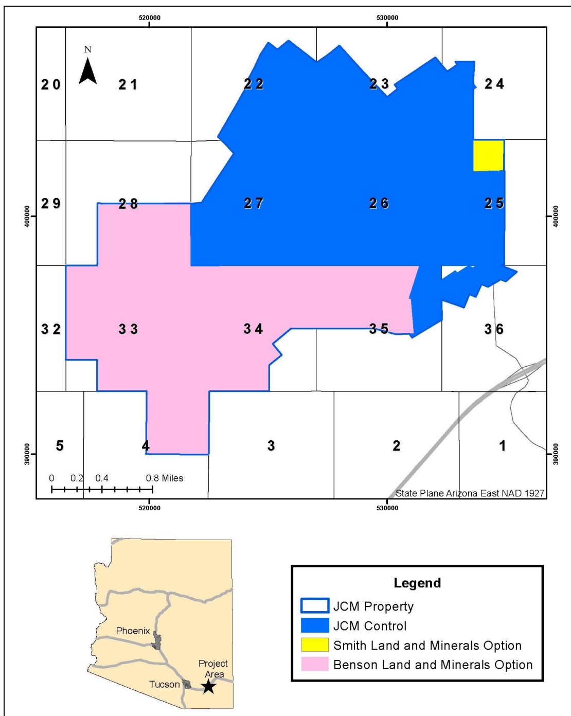
Figure 4-1: Location of the JCM Property – January 2025
