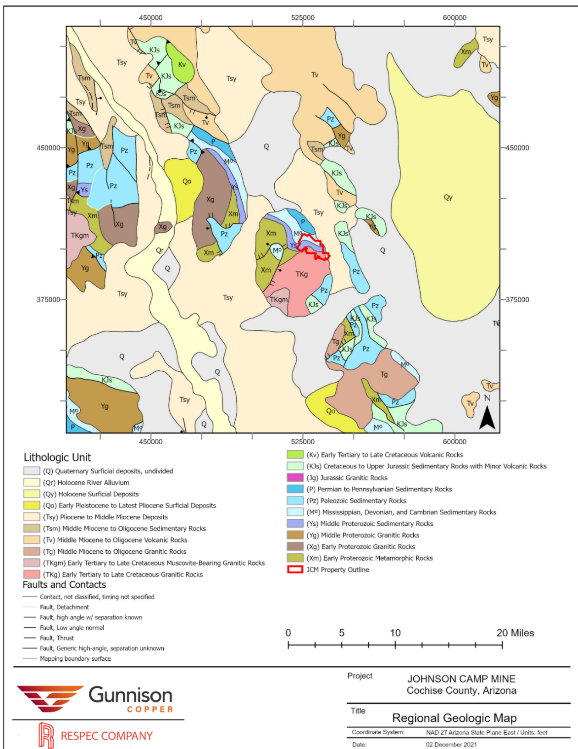
(modified from Richard et al., 2000) Figure 7-1: Regional Geology Little Dagoon Mountains with Historical Boundary
