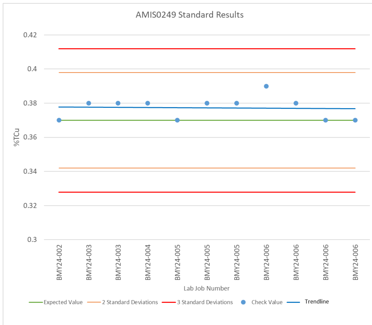
Figure 11-26: 2023 AMIS 0249 Total Copper Analyses
