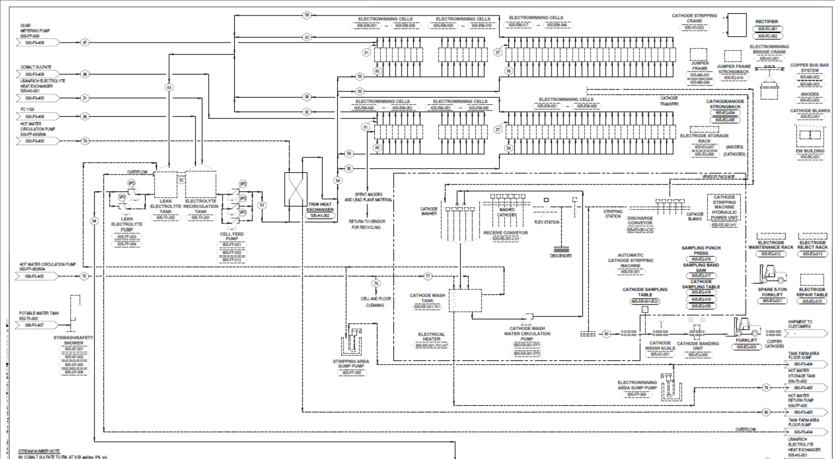
Source: M3, 2016 Figure 17-10: Electrowinning Flowsheet at JCM
